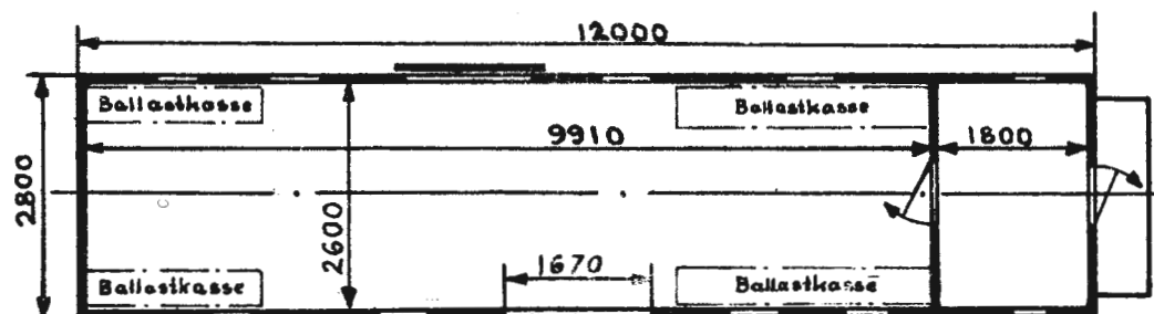
Grunnriss 2
