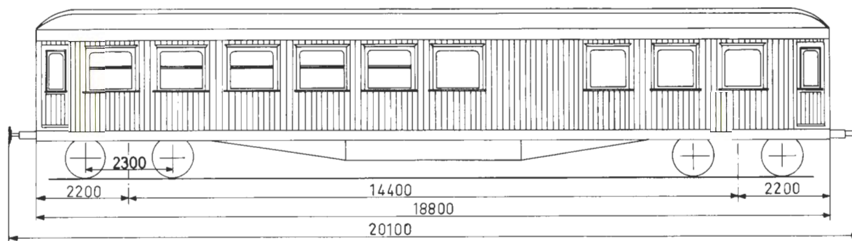
Grunnriss 1
