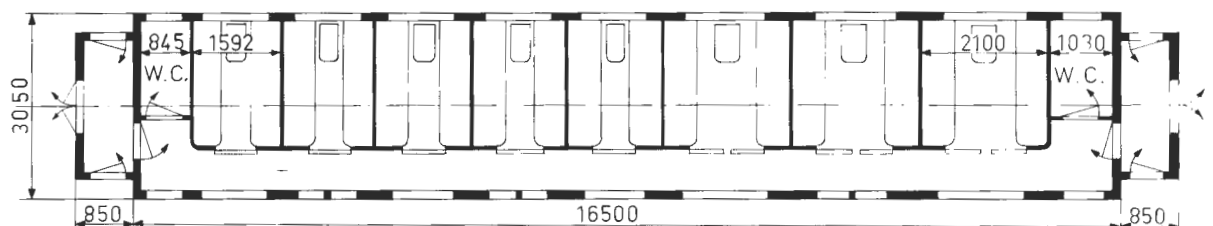
Grunnriss 3
