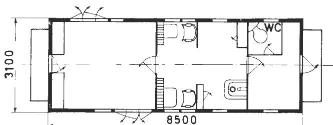
Grunnriss 2
