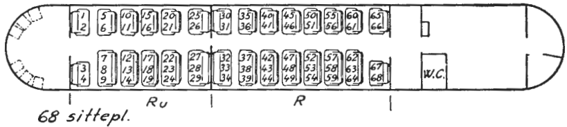
CFox 4b, styrevogn for Cmdo type 6.
