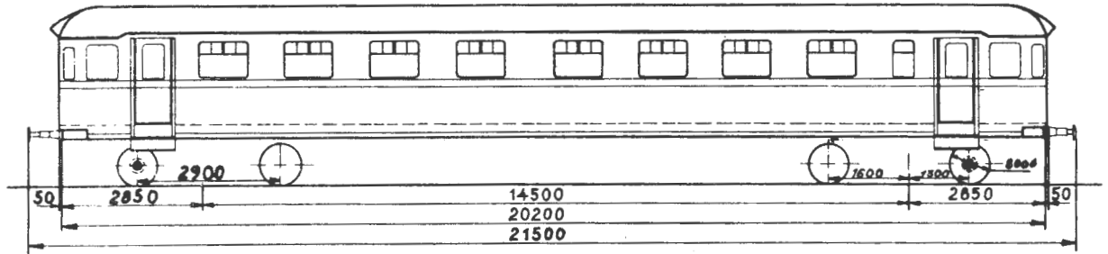
Grunnriss BM 91
