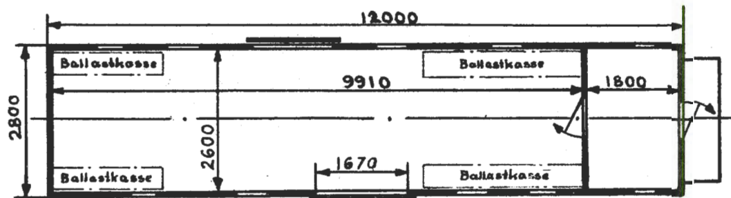
Grunnriss 2
