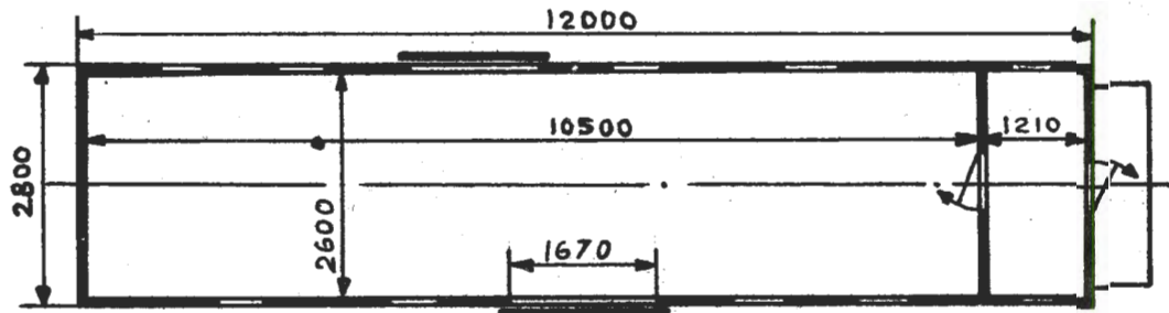
Grunnriss 1
