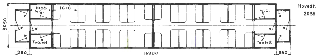
Grunnriss 2
