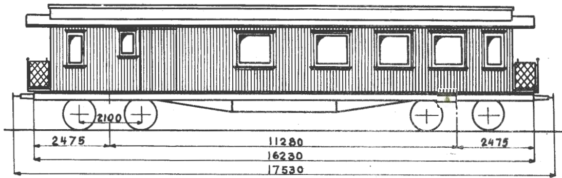
Grunnriss 1
