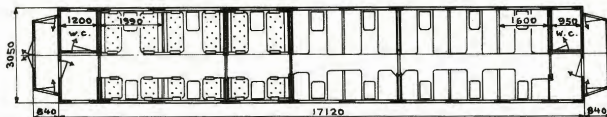
Grunnriss 2
