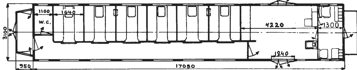
Grunnriss 1
