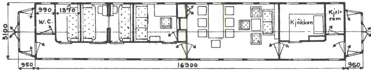
Grunnriss 2
