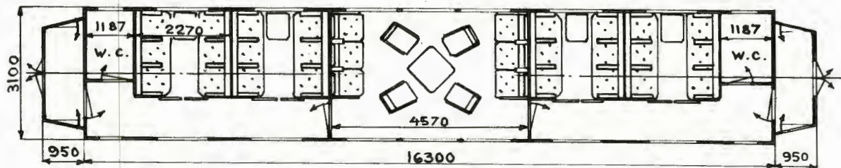
Grunnriss 2
