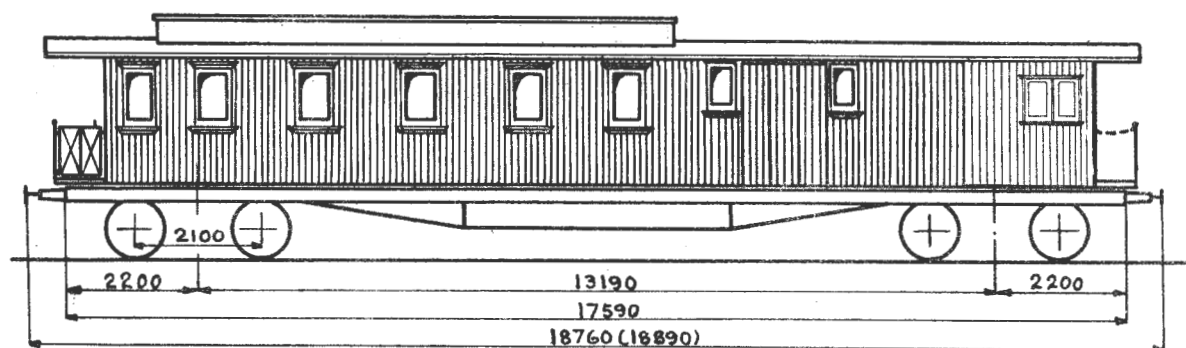
Grunnriss 1
