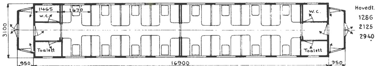
Grunnriss 1
