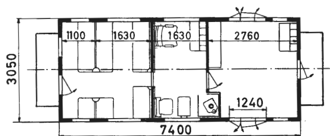
Grunnriss 2 1)
