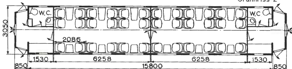
Grunnriss 2
