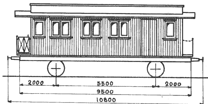
Grunnriss 1
