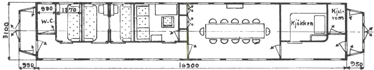
Grunnriss 1
