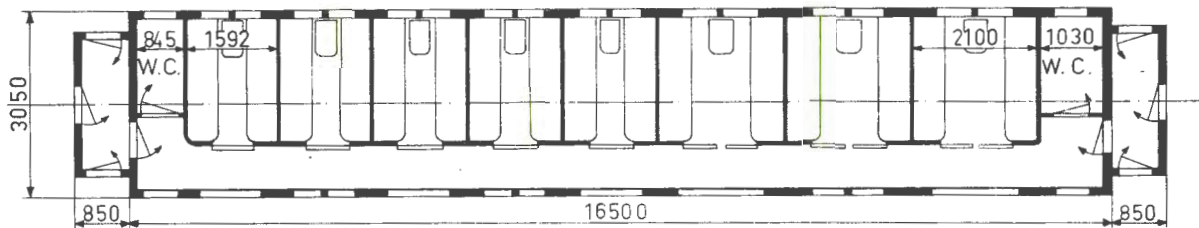
Grunnriss 2
