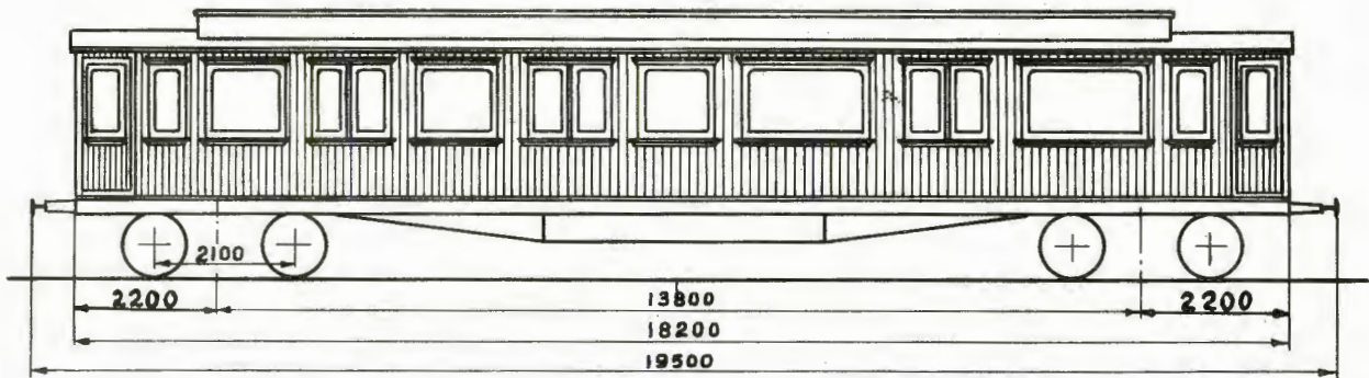
Grunnriss 1
