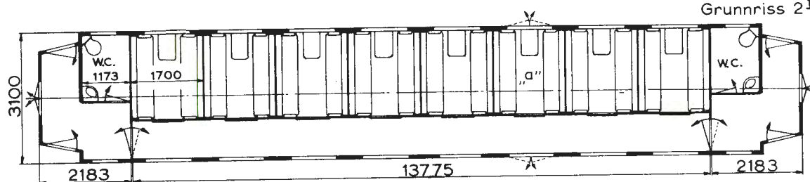
Grunnriss 2 ↓
