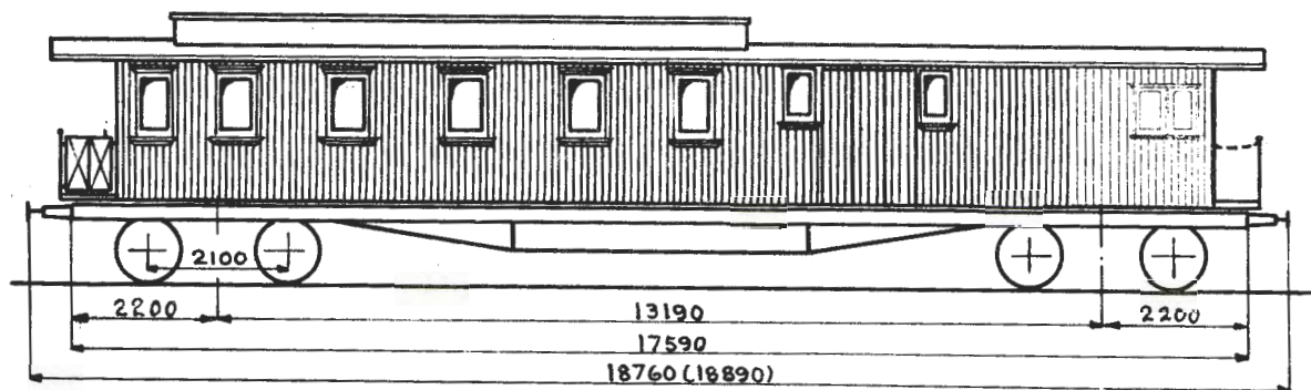
Grunnriss 1
