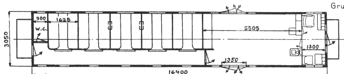
Grunnriss 2
