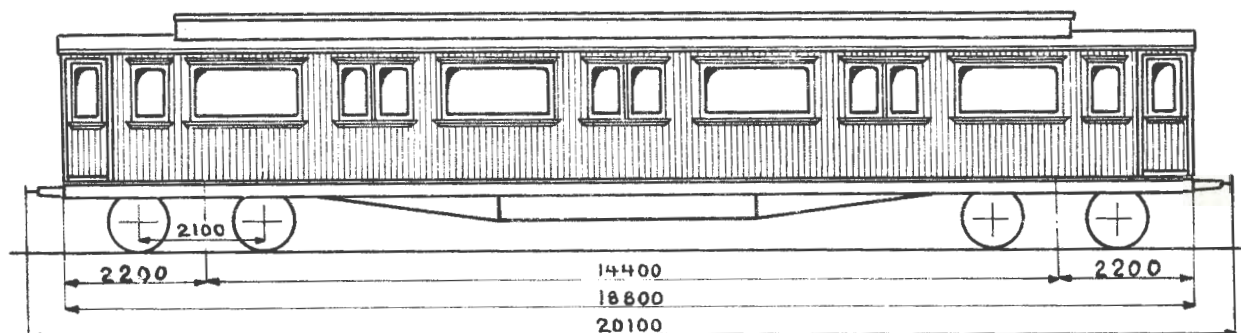
Grunnriss 1
