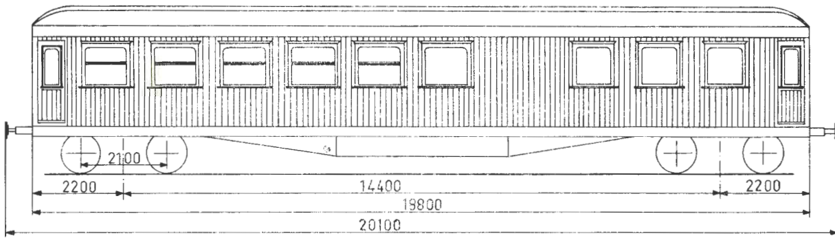
Grunnriss 1
