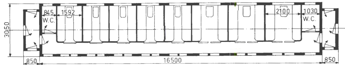
Grunnriss 3
