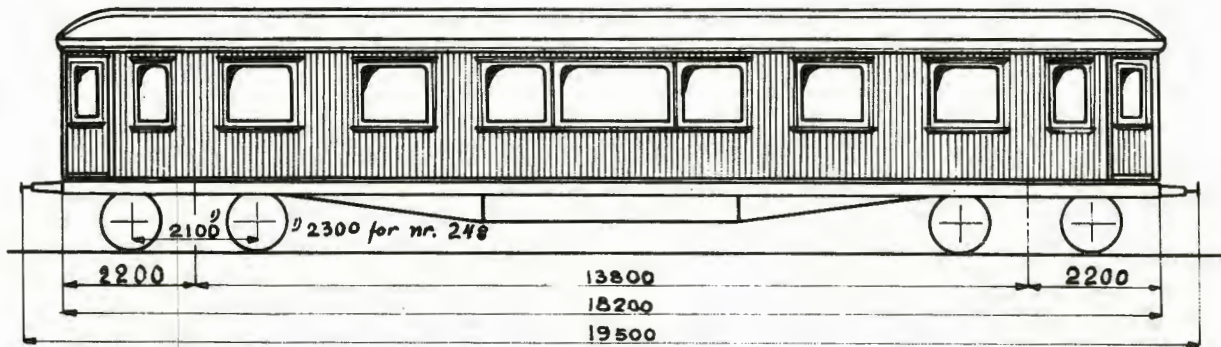
Grunnriss 1
