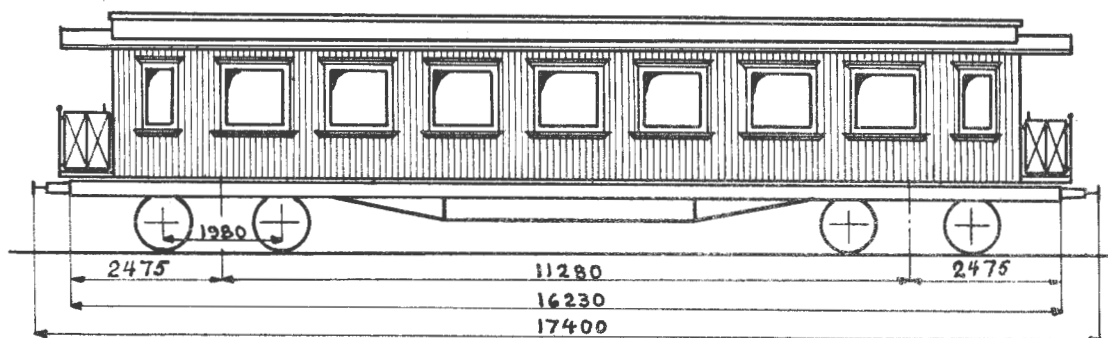
Grunnriss 1
